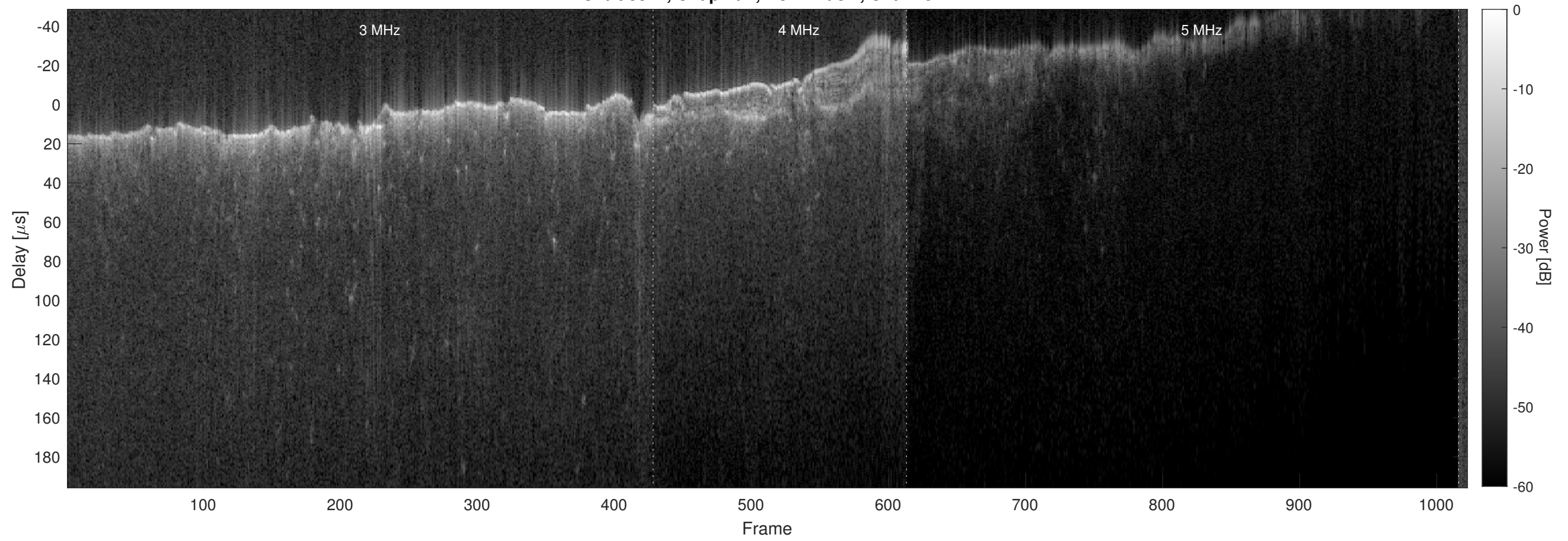
Orbit 8814, Chapman, No Window, Channel 2
