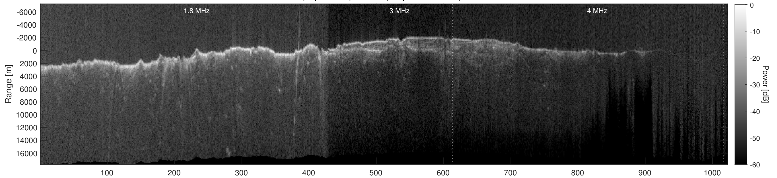
Orbit 8814, Depth-Corrected Cluttergram
