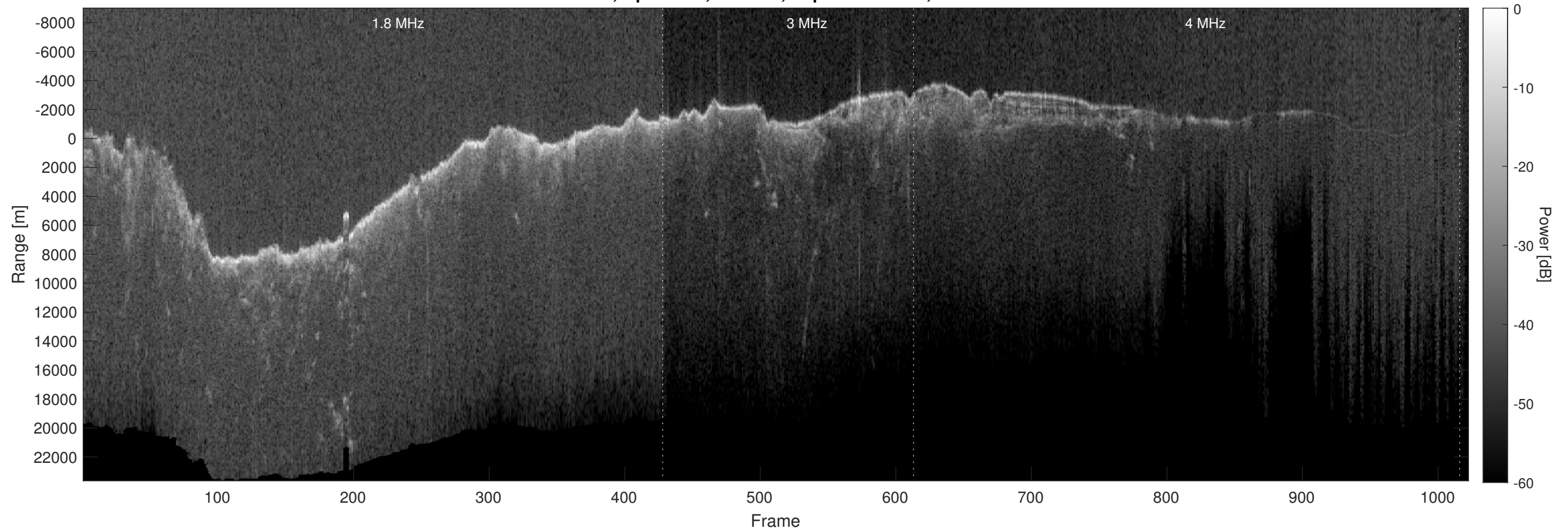
Orbit 8815, Optimized, Window, Depth-Corrected, Channel 2
