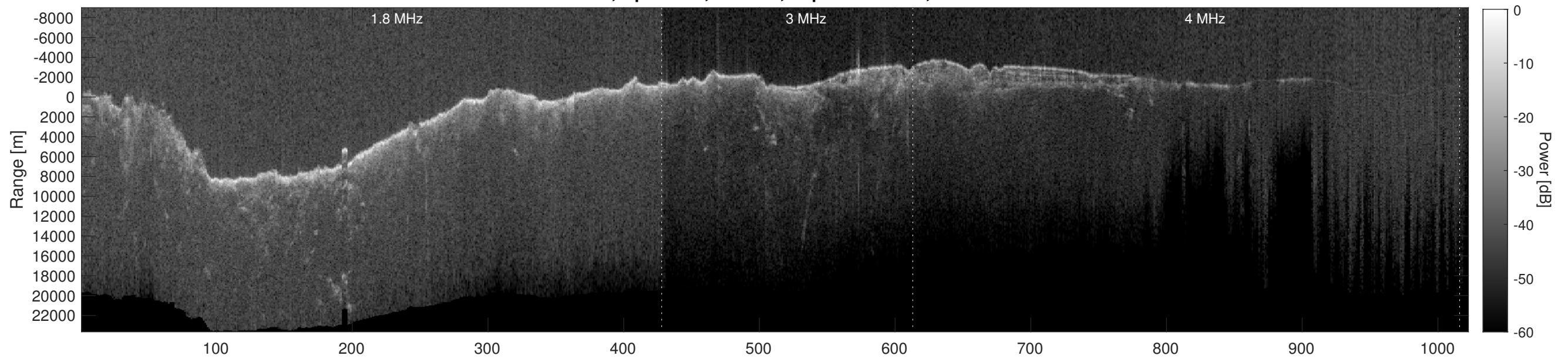
Orbit 8815, Depth-Corrected Cluttergram
