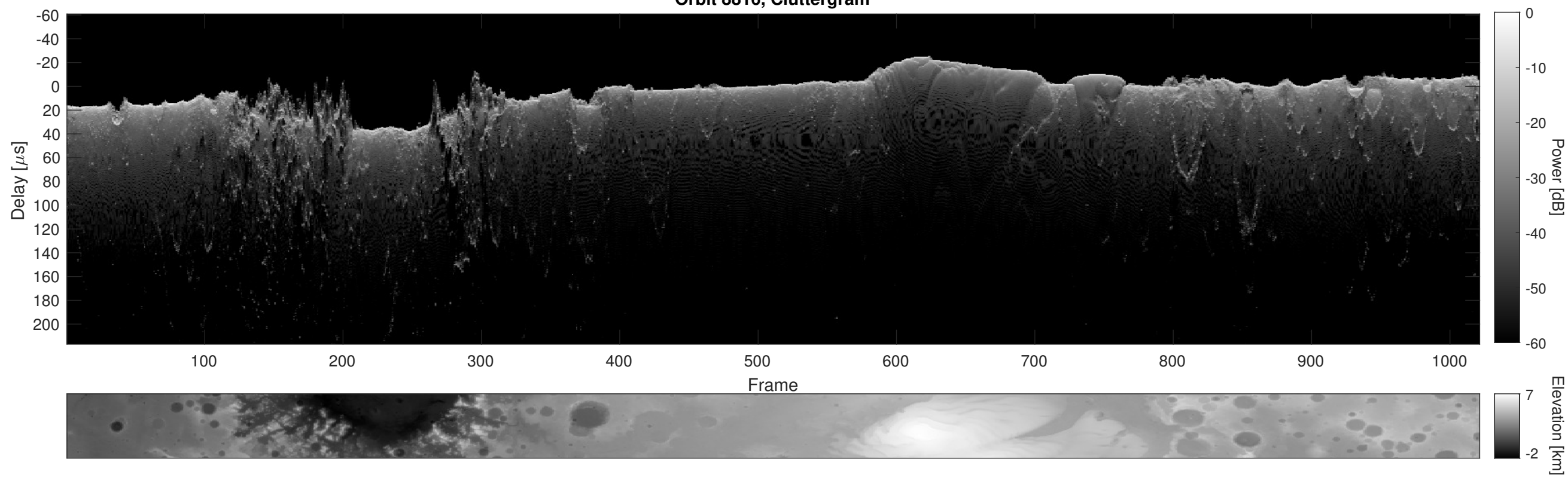
Orbit 8816, Cluttergram
