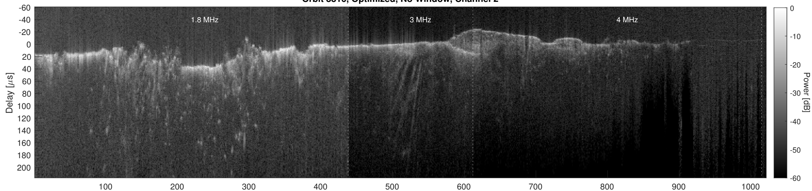
Orbit 8816, Cluttergram
