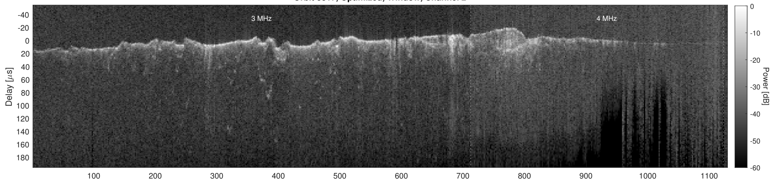
Orbit 8817, Cluttergram
