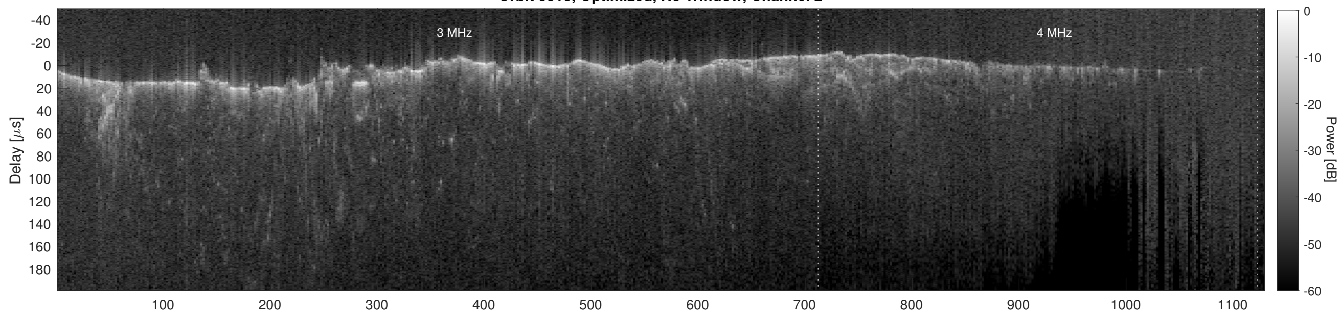
Orbit 8818, Cluttergram
