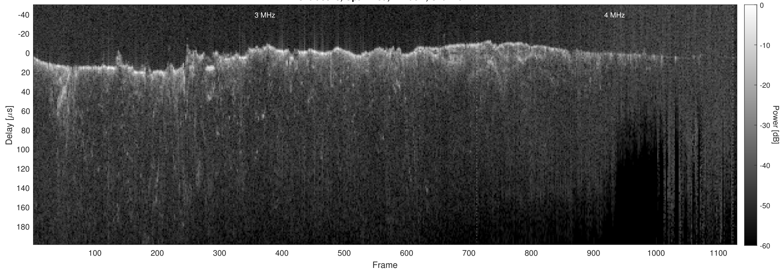
Orbit 8818, Optimized, Window, Channel 2
