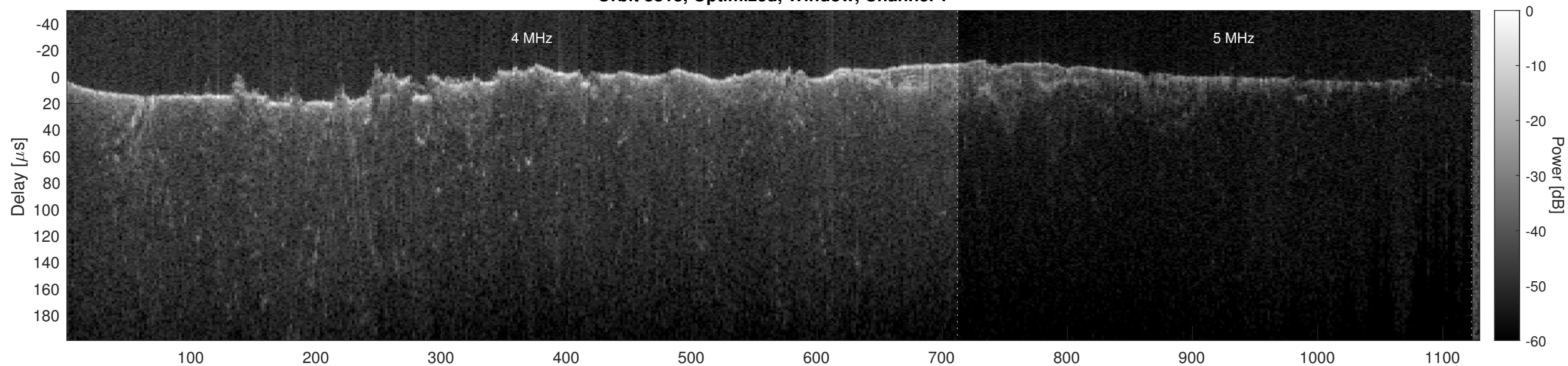
Orbit 8818, Optimized, Window, Channel 2
