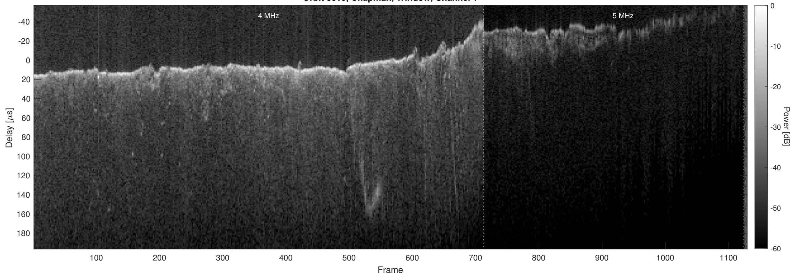
Orbit 8819, Chapman, Window, Channel 2
