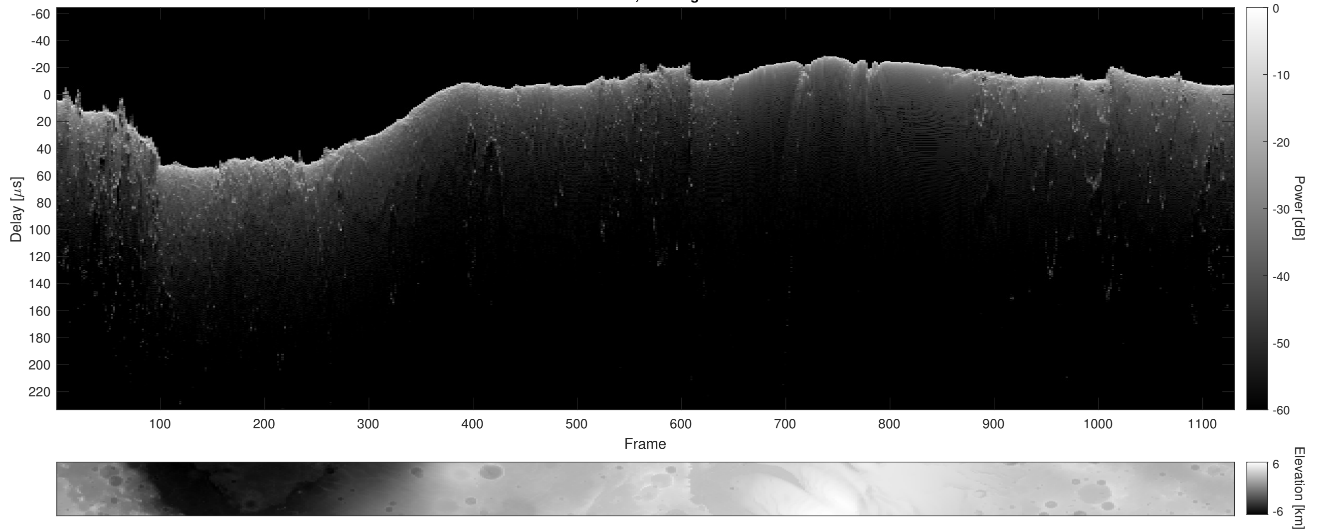
Orbit 8822, Cluttergram
