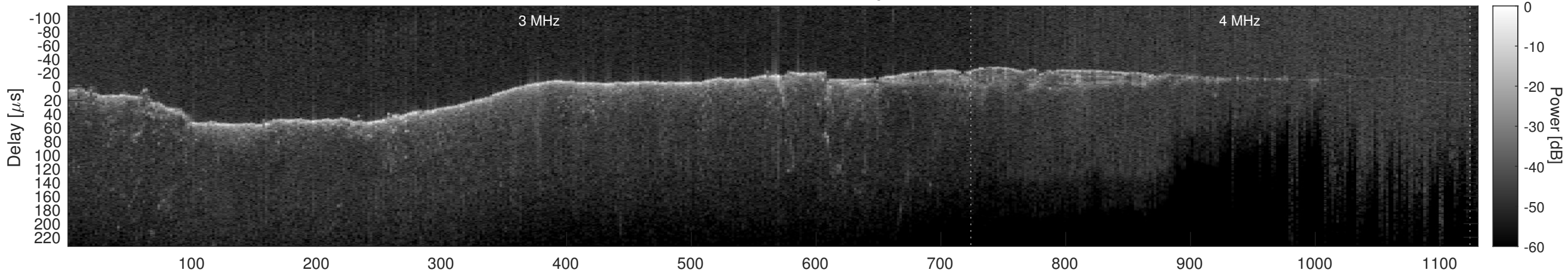
Orbit 8822, Cluttergram
