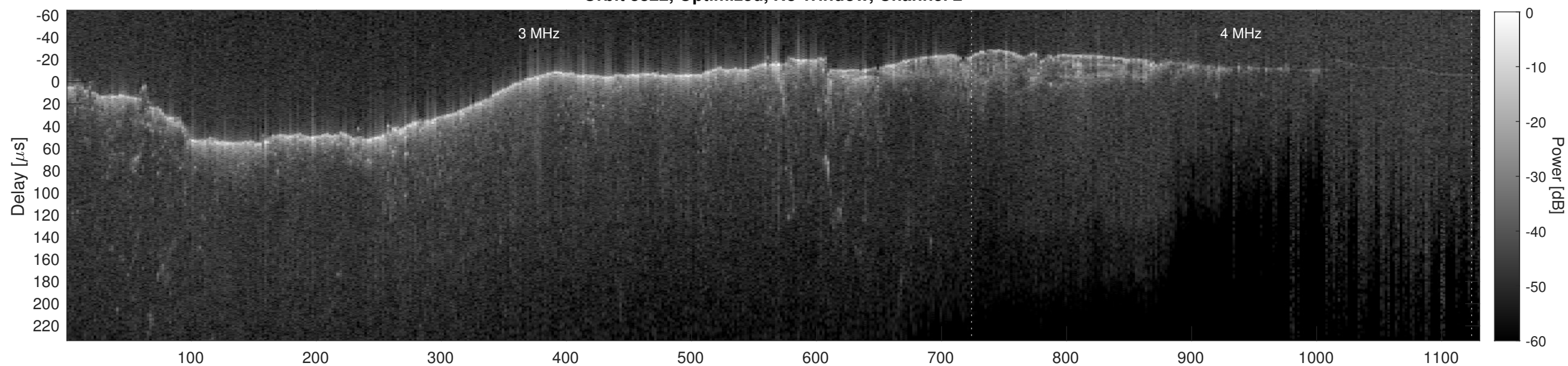
Orbit 8822, Cluttergram
