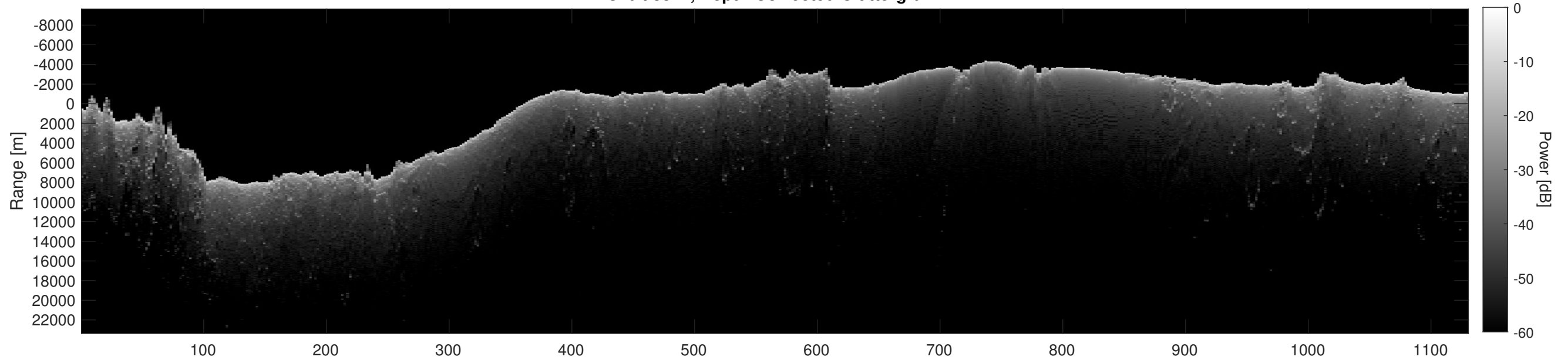
Orbit 8822, Depth-Corrected Cluttergram
