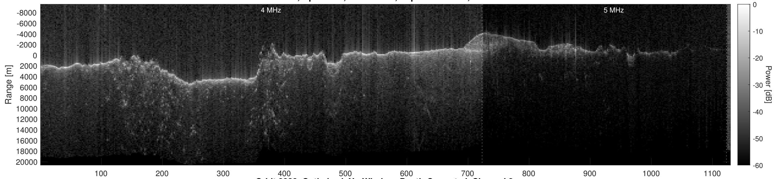
Orbit 8823, Optimized, No Window, Depth-Corrected, Channel 2
