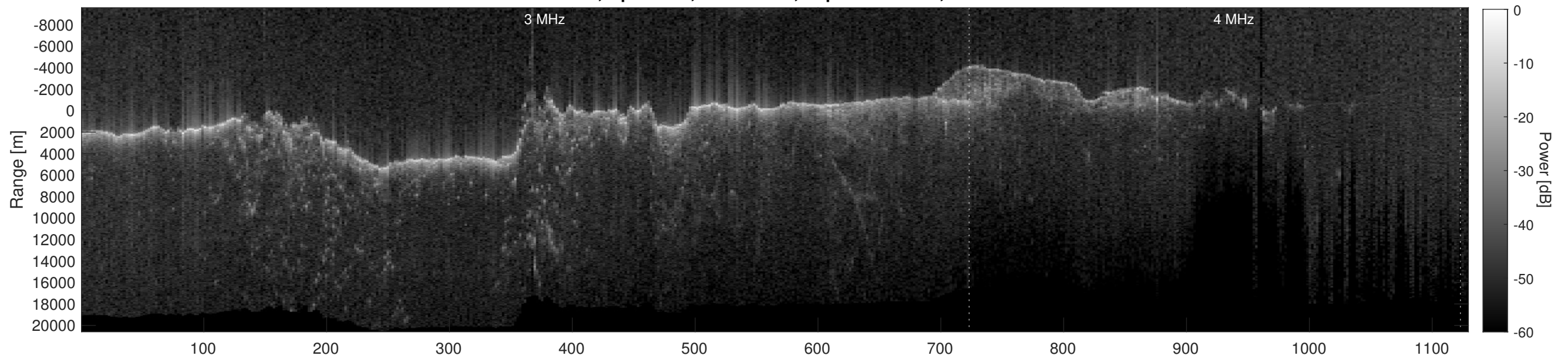
Orbit 8823, Depth-Corrected Cluttergram
