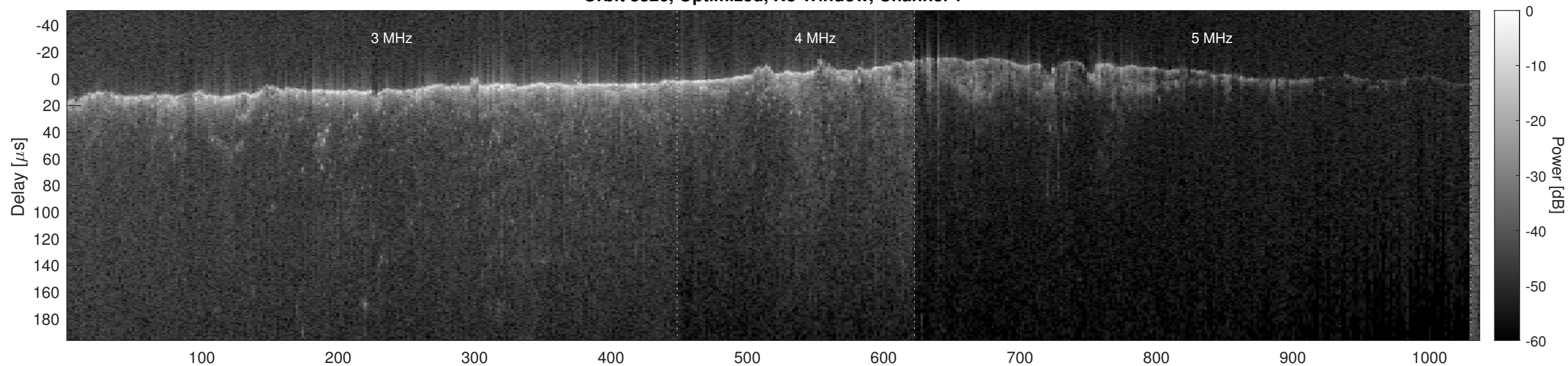
Orbit 8826, Optimized, No Window, Channel 2
