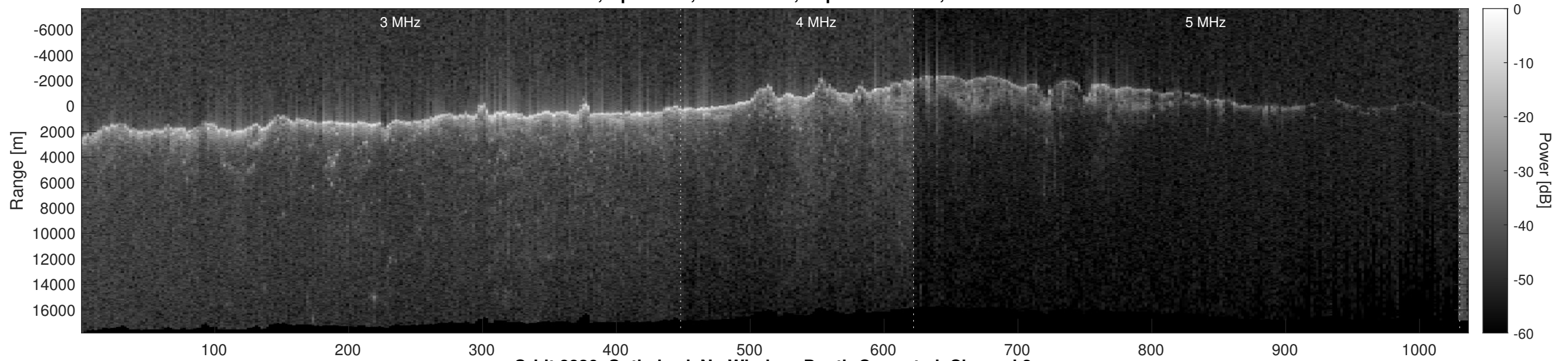
Orbit 8826, Optimized, No Window, Depth-Corrected, Channel 2
