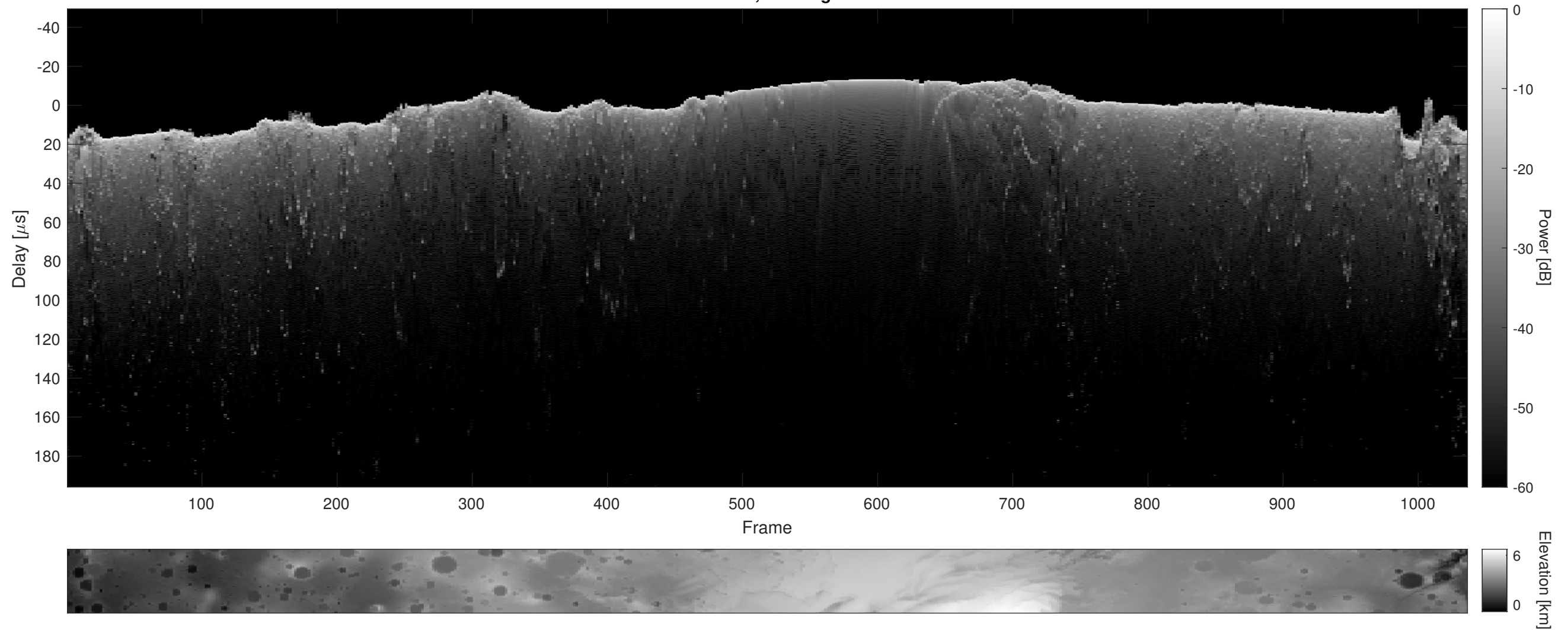
Orbit 8828, Cluttergram
