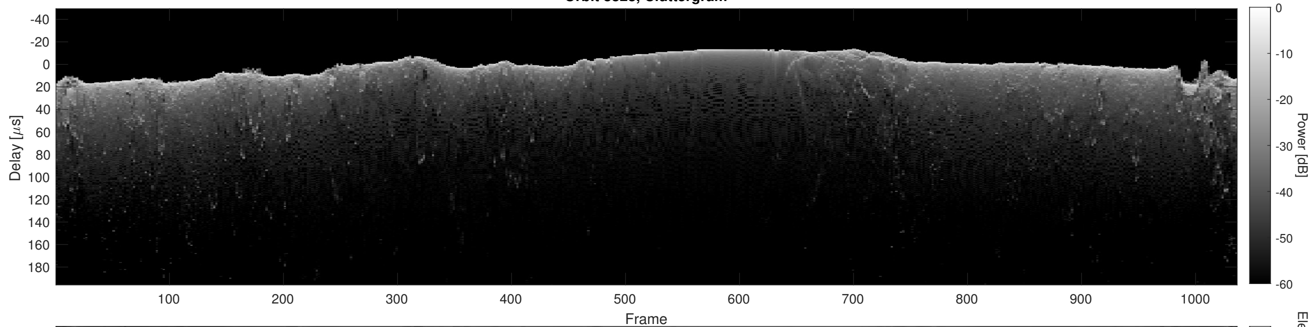
Orbit 8828, Cluttergram
