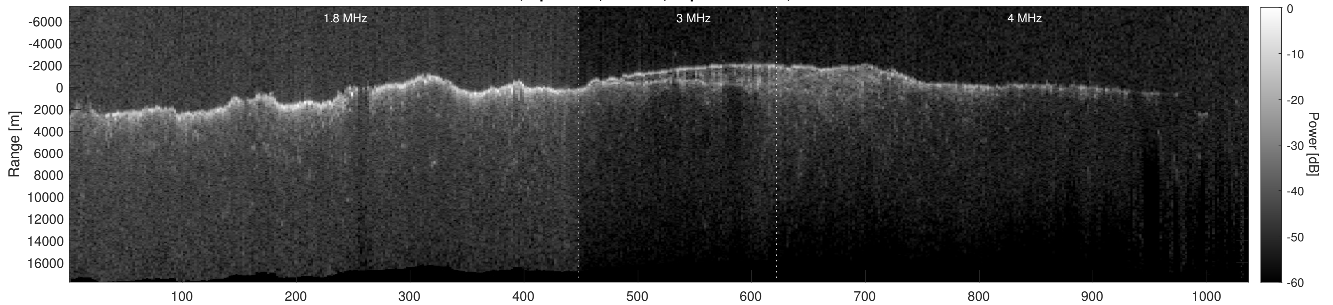
Orbit 8828, Depth-Corrected Cluttergram
