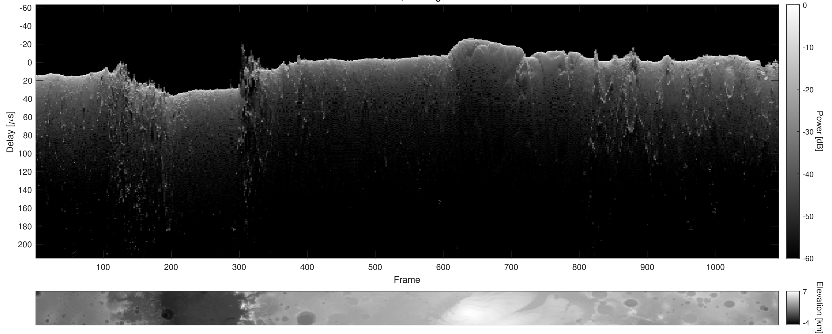
Orbit 8830, Cluttergram
