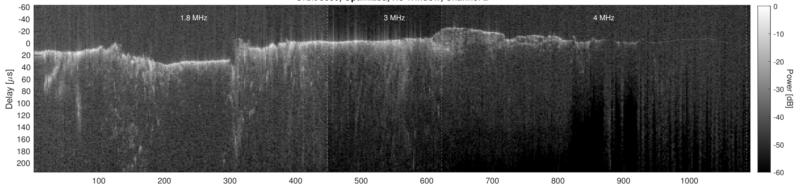
Orbit 8830, Cluttergram
