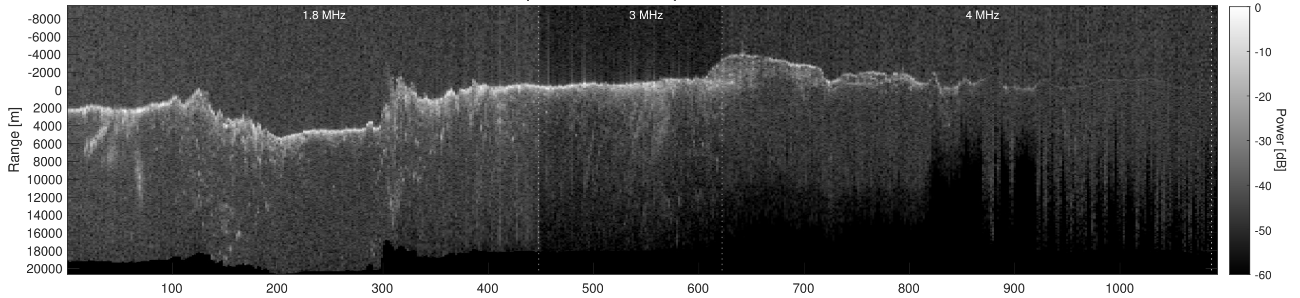
Orbit 8830, Depth-Corrected Cluttergram
