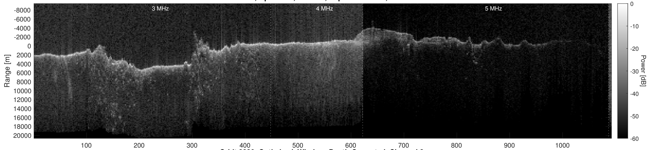
Orbit 8830, Optimized, Window, Depth-Corrected, Channel 2
