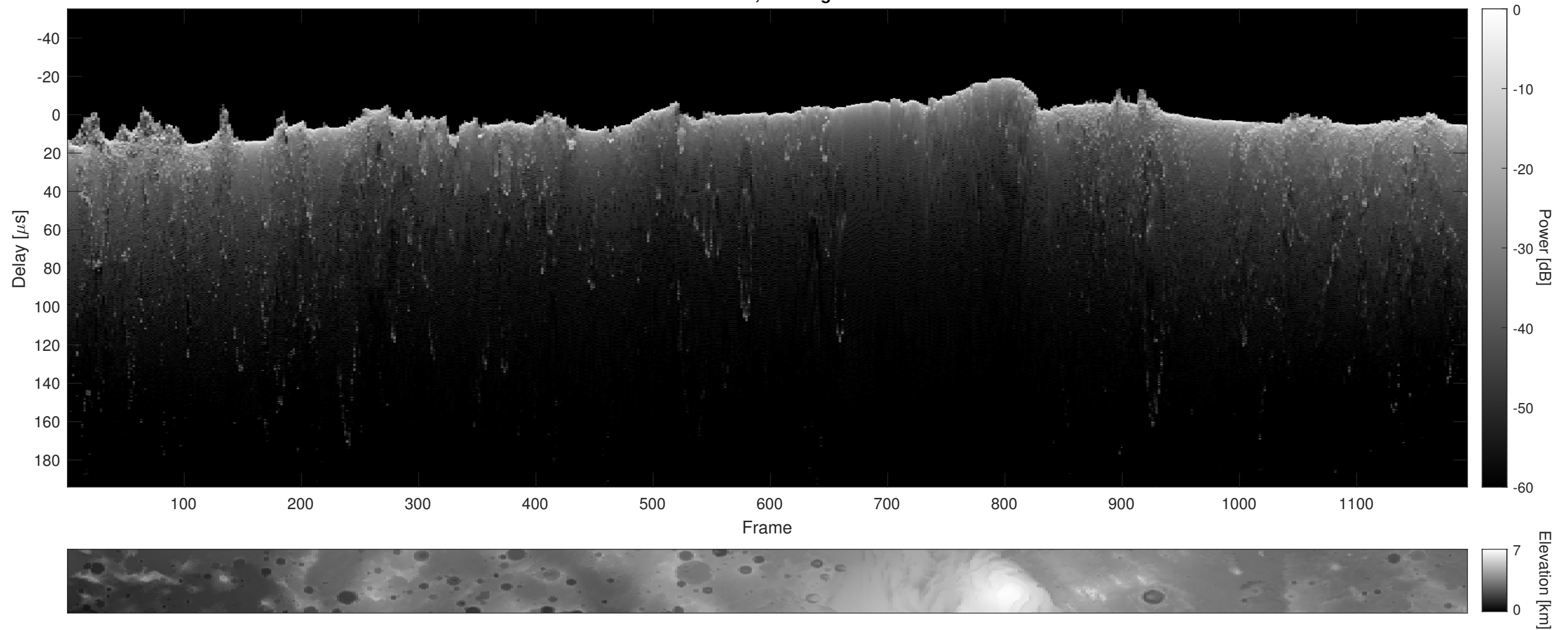
Orbit 8831, Cluttergram
