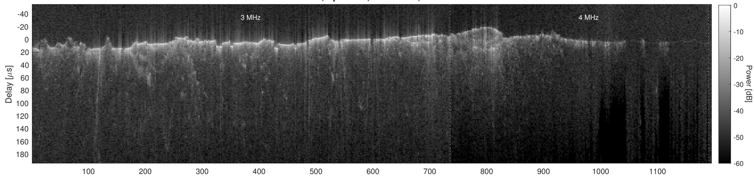
Orbit 8831, Cluttergram
