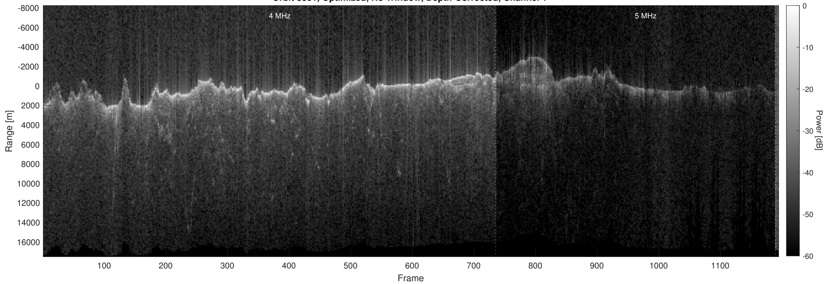
Orbit 8831, Optimized, No Window, Depth-Corrected, Channel 2
