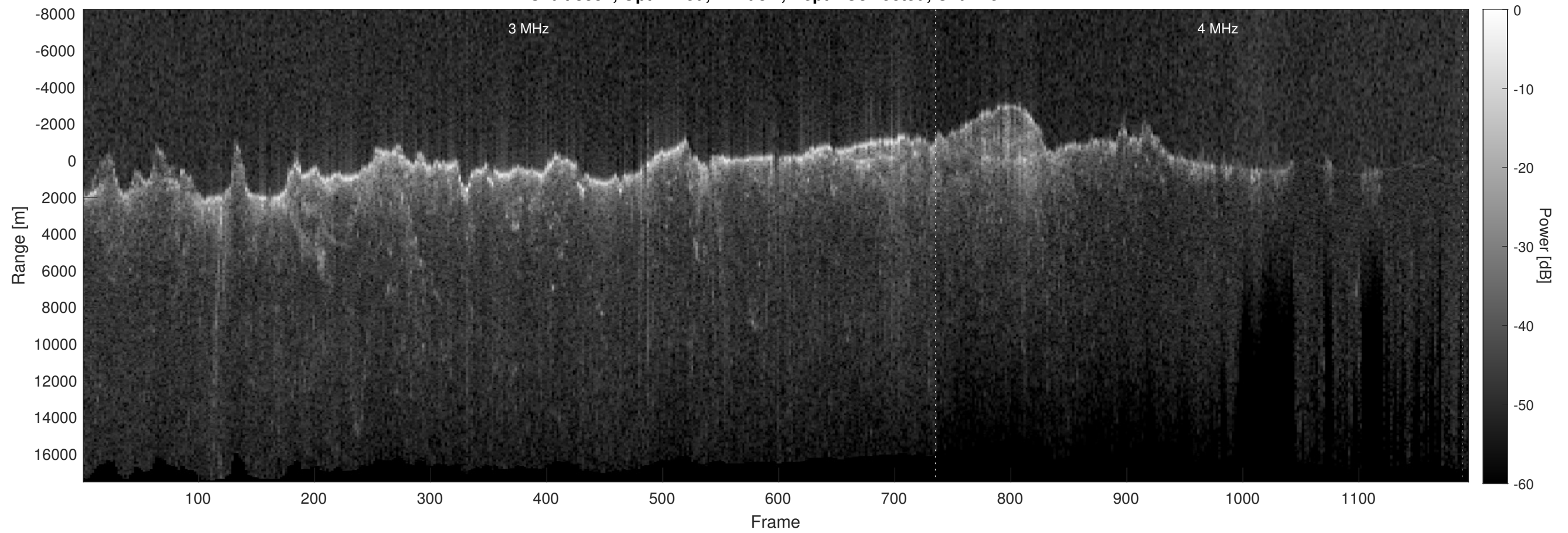
Orbit 8831, Optimized, Window, Depth-Corrected, Channel 2
