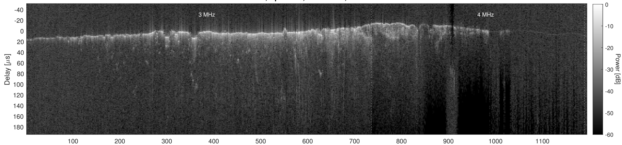
Orbit 8833, Cluttergram
