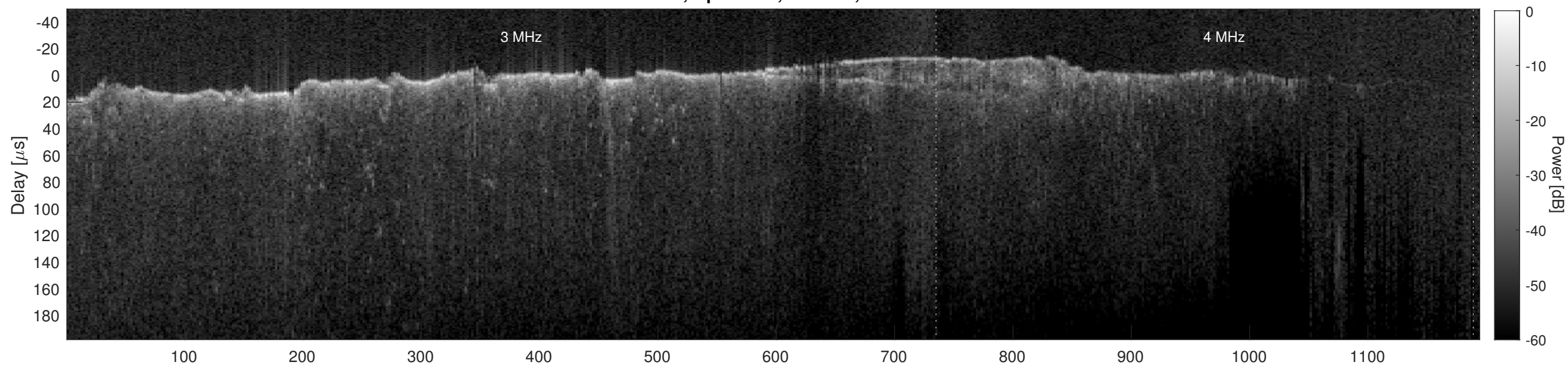
Orbit 8835, Cluttergram
