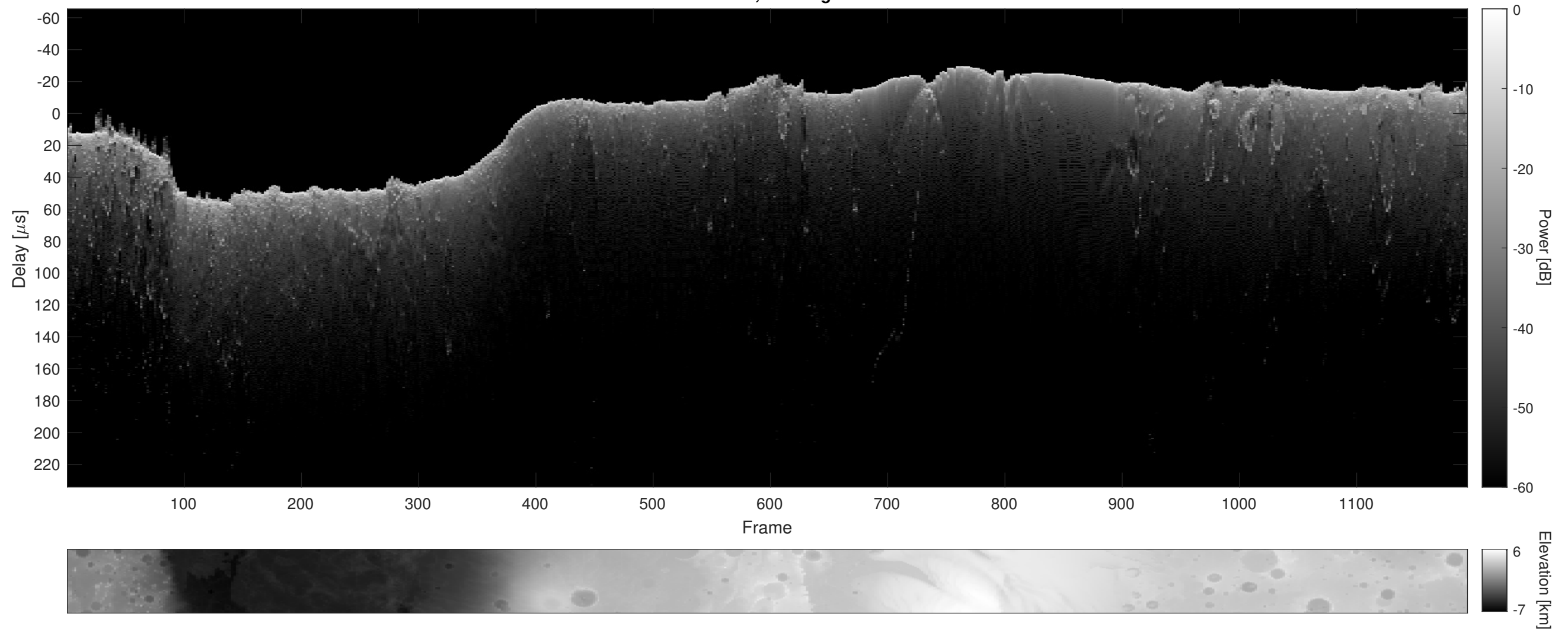
Orbit 8836, Cluttergram
