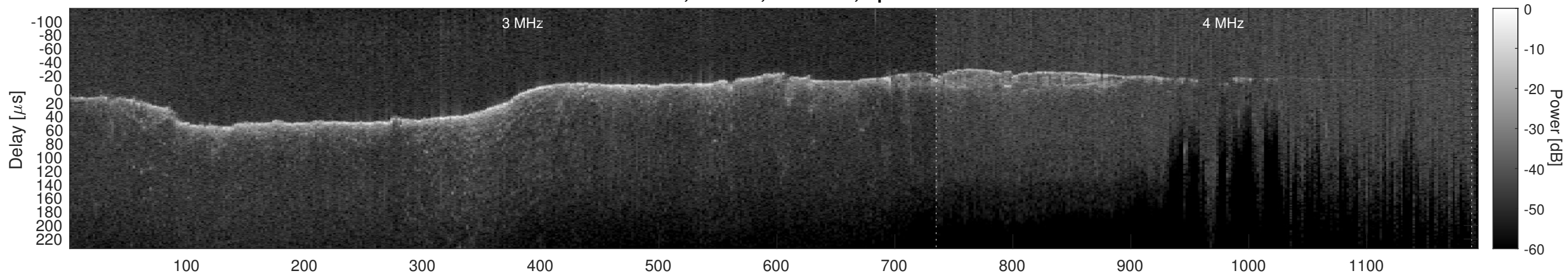
Orbit 8836, Cluttergram
