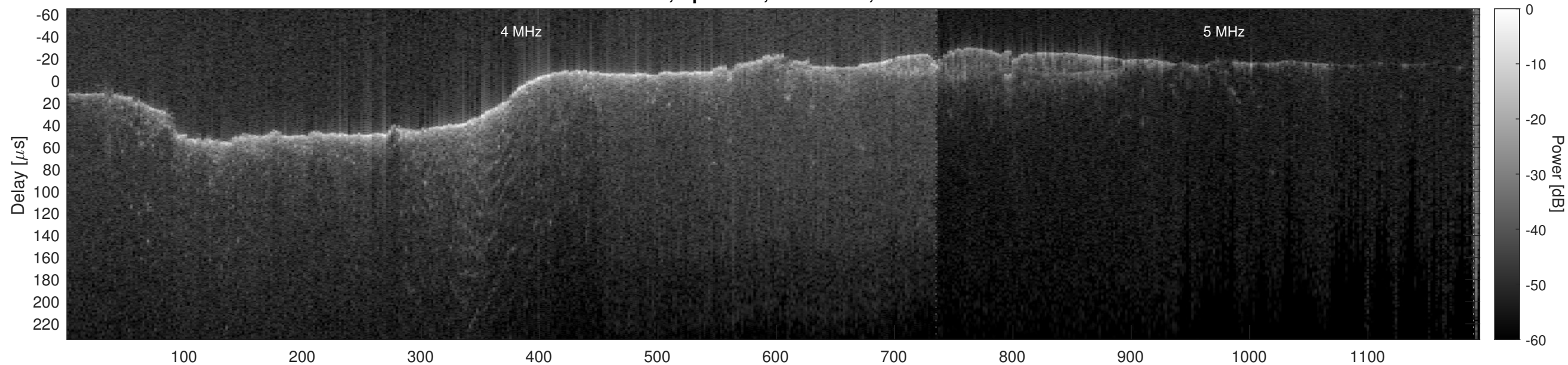
Orbit 8836, Optimized, No Window, Channel 2
