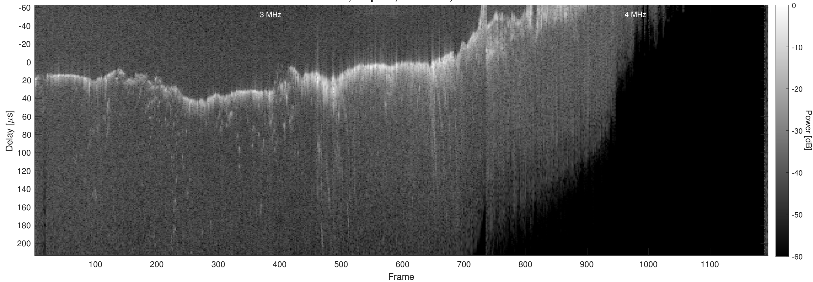
Orbit 8837, Chapman, No Window, Channel 2
