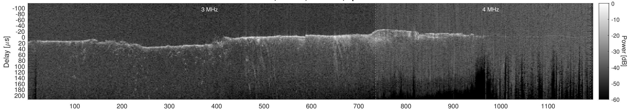
Orbit 8837, Cluttergram
