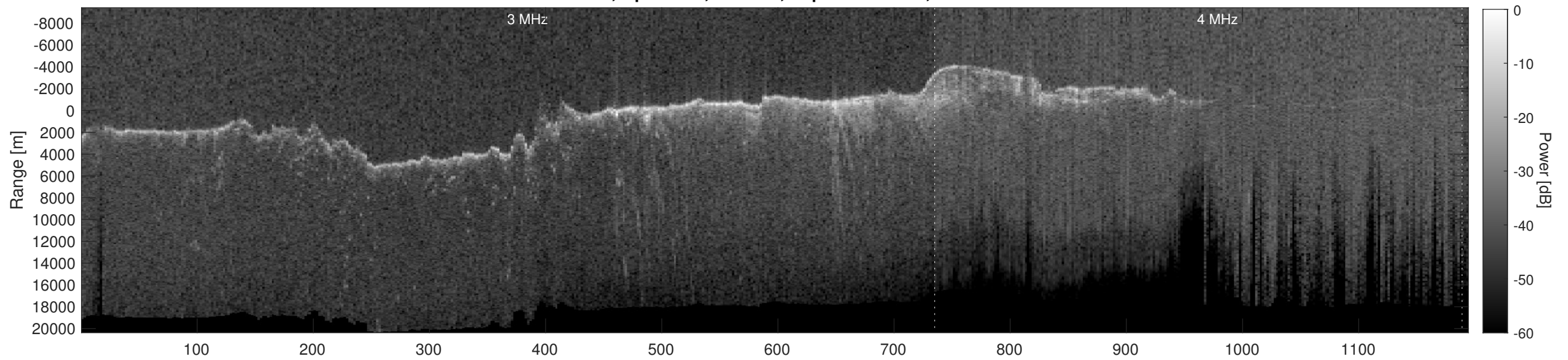
Orbit 8837, Depth-Corrected Cluttergram
