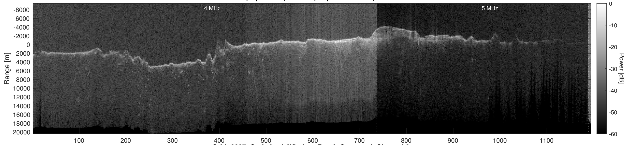
Orbit 8837, Optimized, Window, Depth-Corrected, Channel 2
