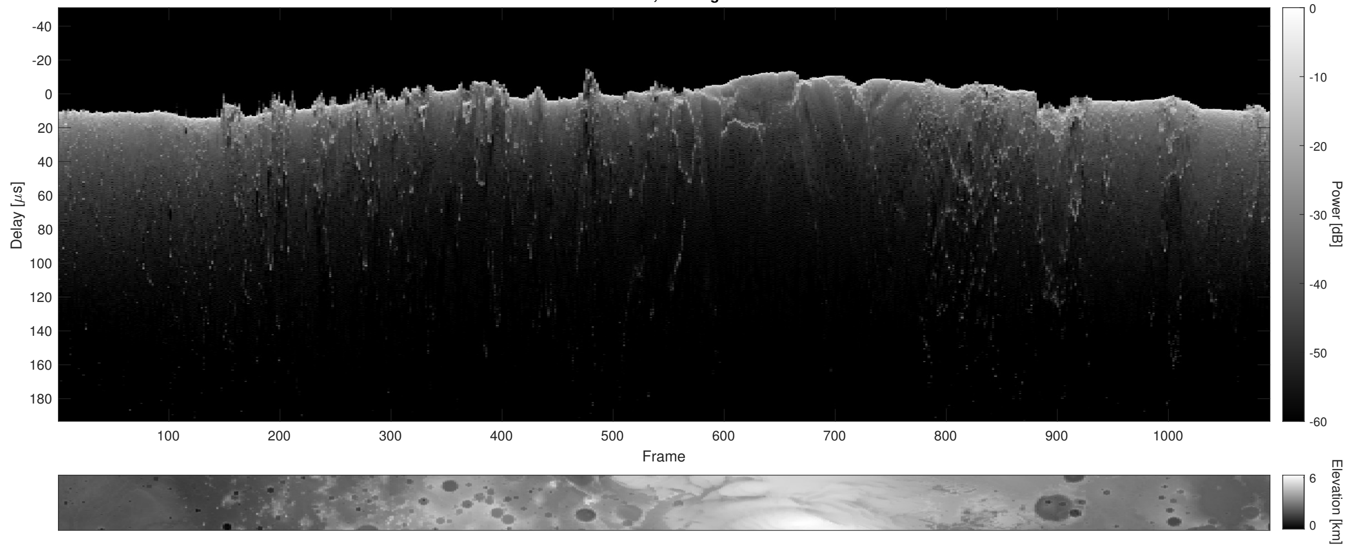
Orbit 8839, Cluttergram
