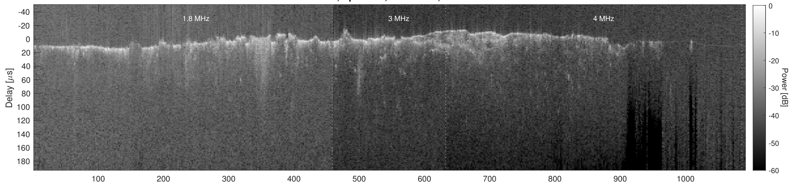
Orbit 8839, Cluttergram
