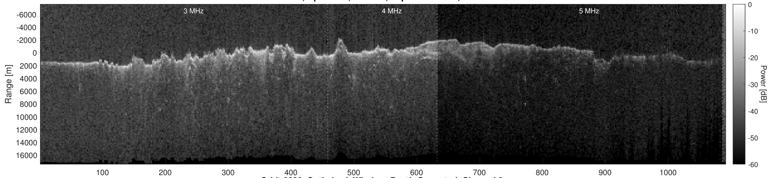
Orbit 8839, Optimized, Window, Depth-Corrected, Channel 2
