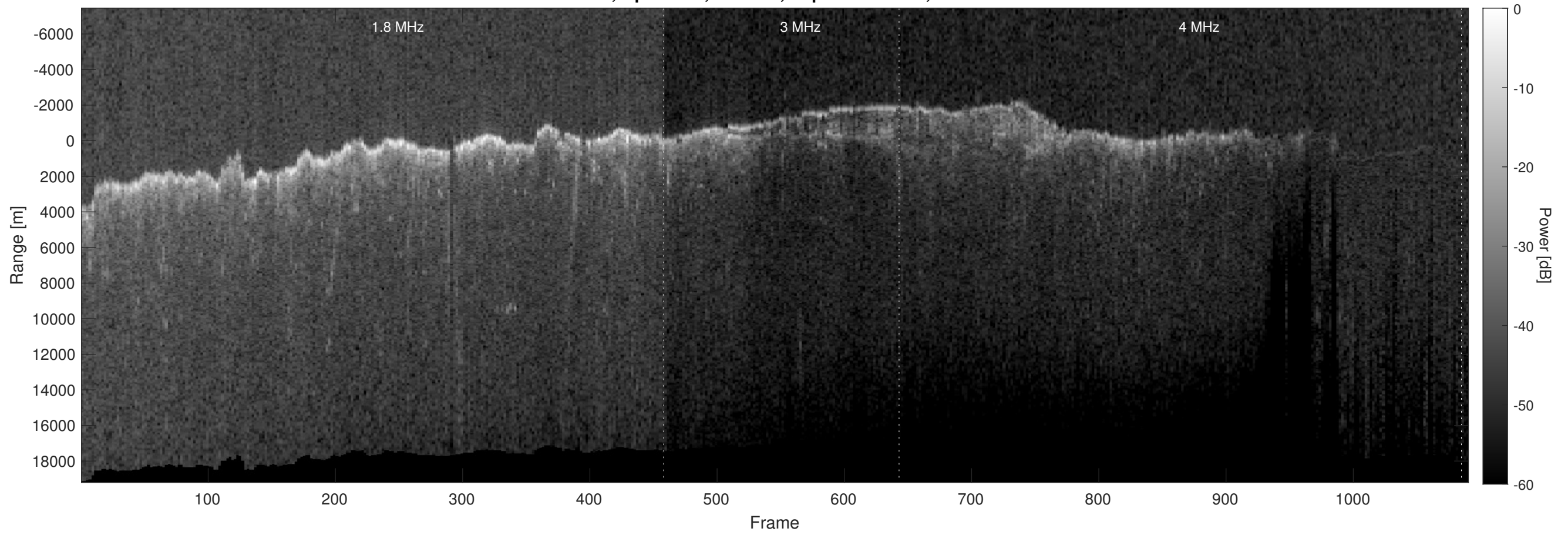
Orbit 8842, Optimized, Window, Depth-Corrected, Channel 2
