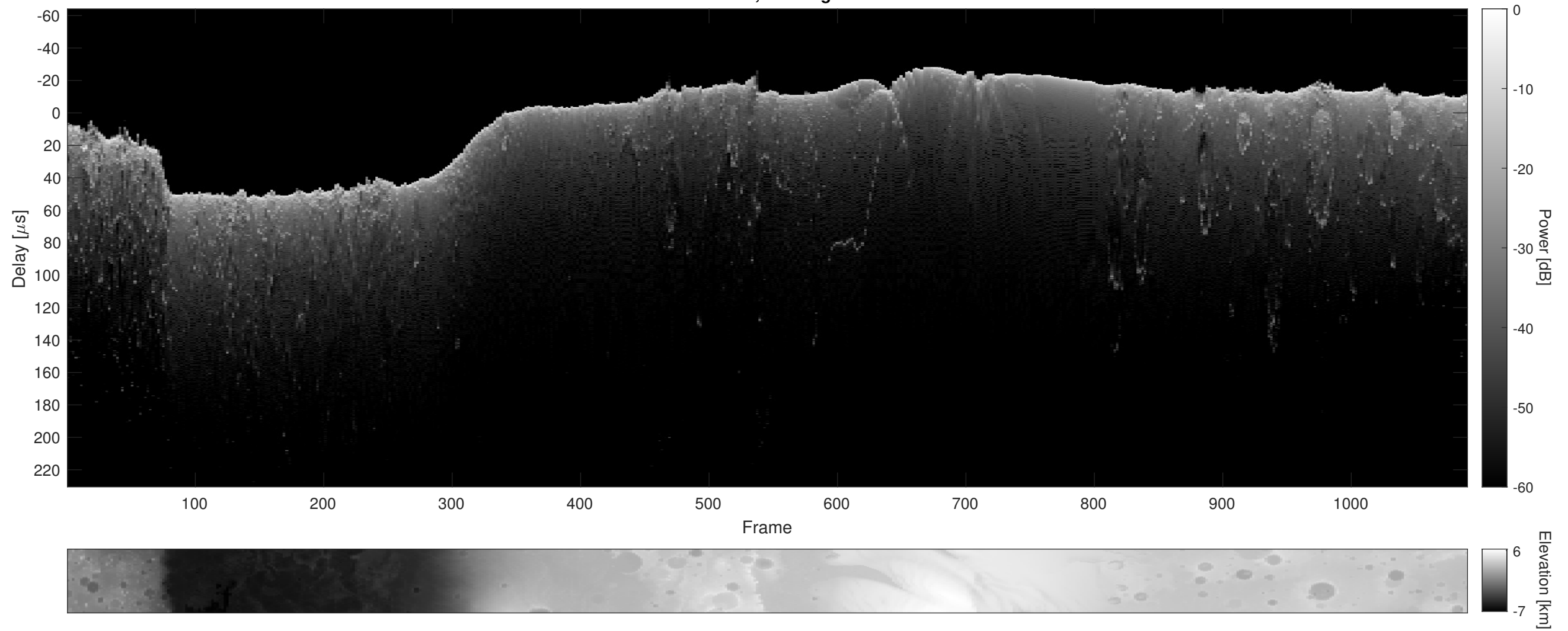
Orbit 8843, Cluttergram
