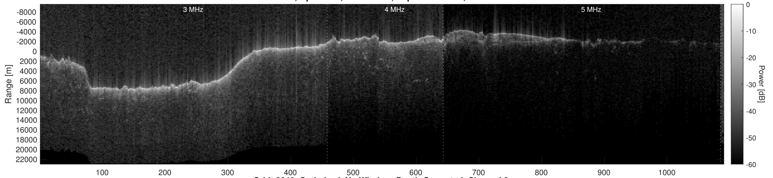
Orbit 8843, Optimized, No Window, Depth-Corrected, Channel 2
