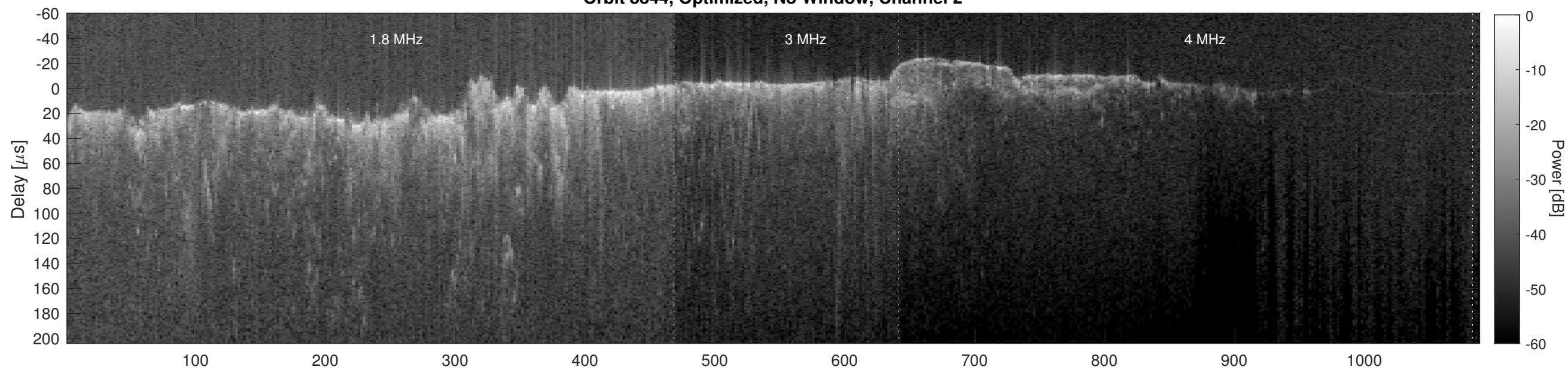
Orbit 8844, Cluttergram
