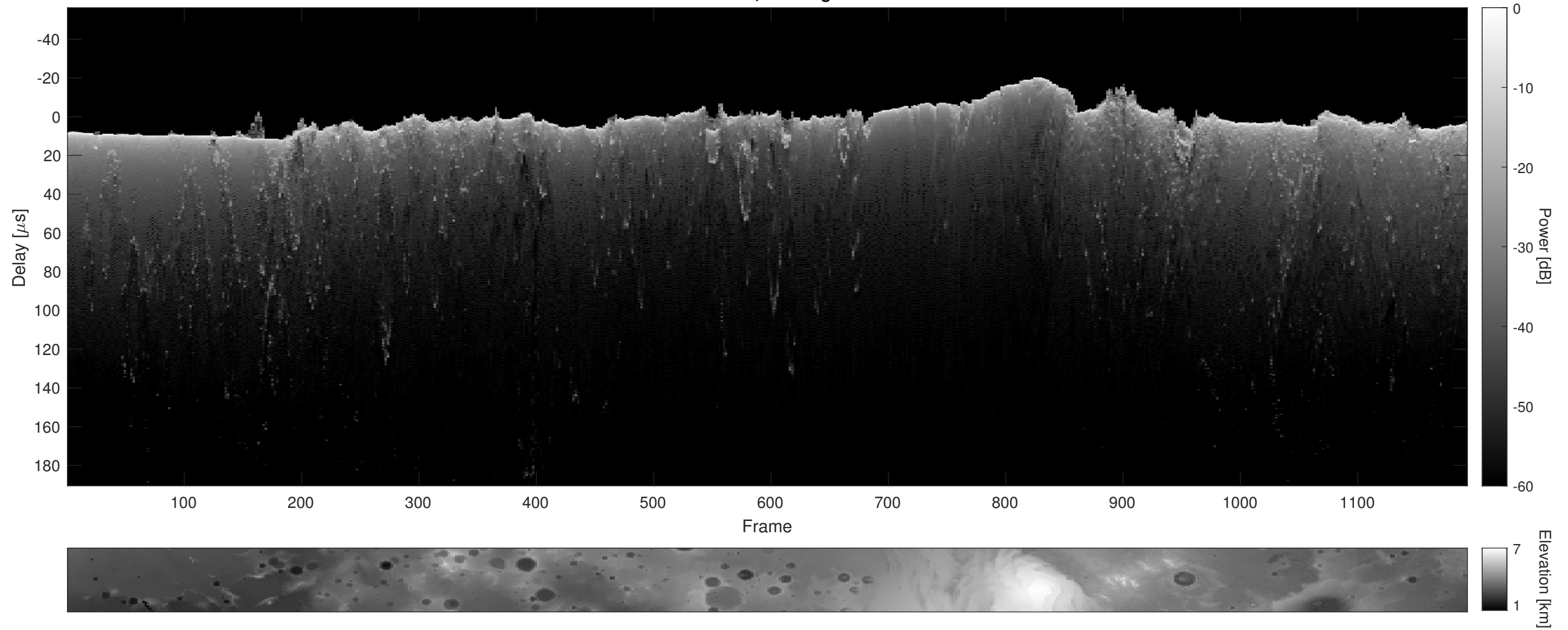
Orbit 8845, Cluttergram
