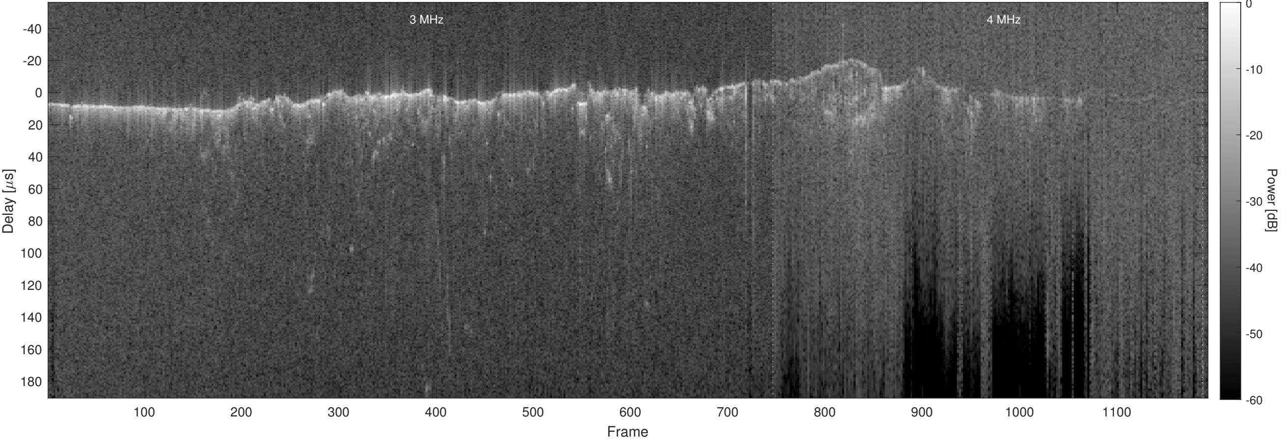
Orbit 8845, Optimized, No Window, Channel 2
