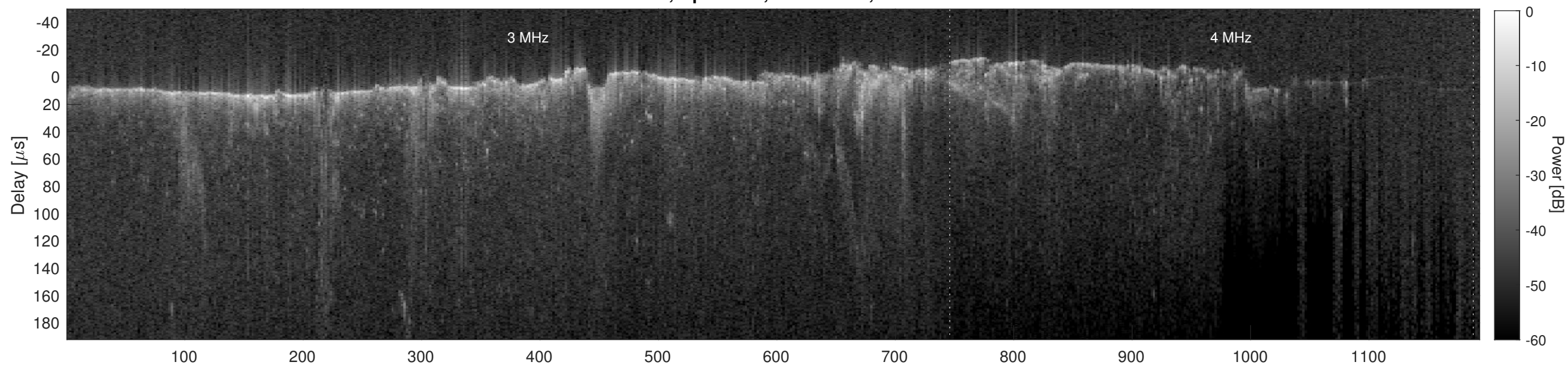
Orbit 8846, Cluttergram
