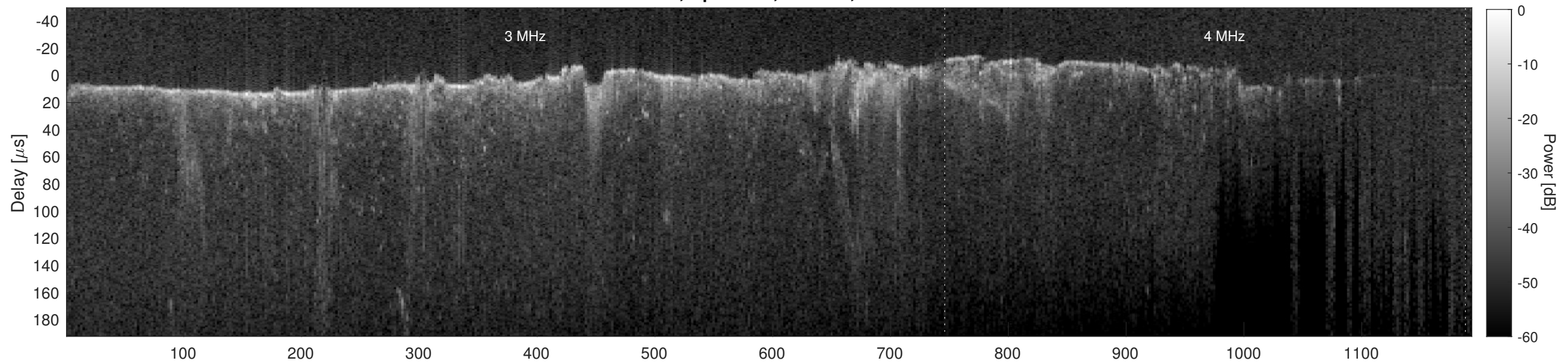
Orbit 8846, Cluttergram
