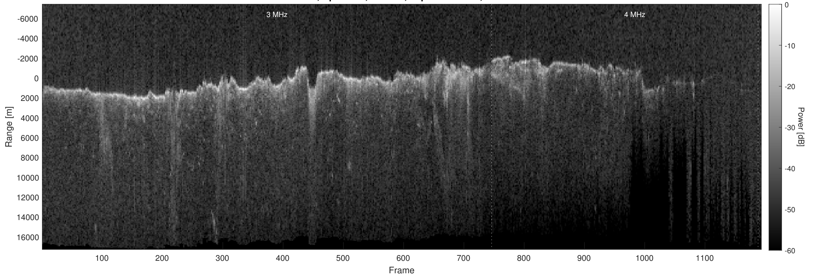
Orbit 8846, Optimized, Window, Depth-Corrected, Channel 2
