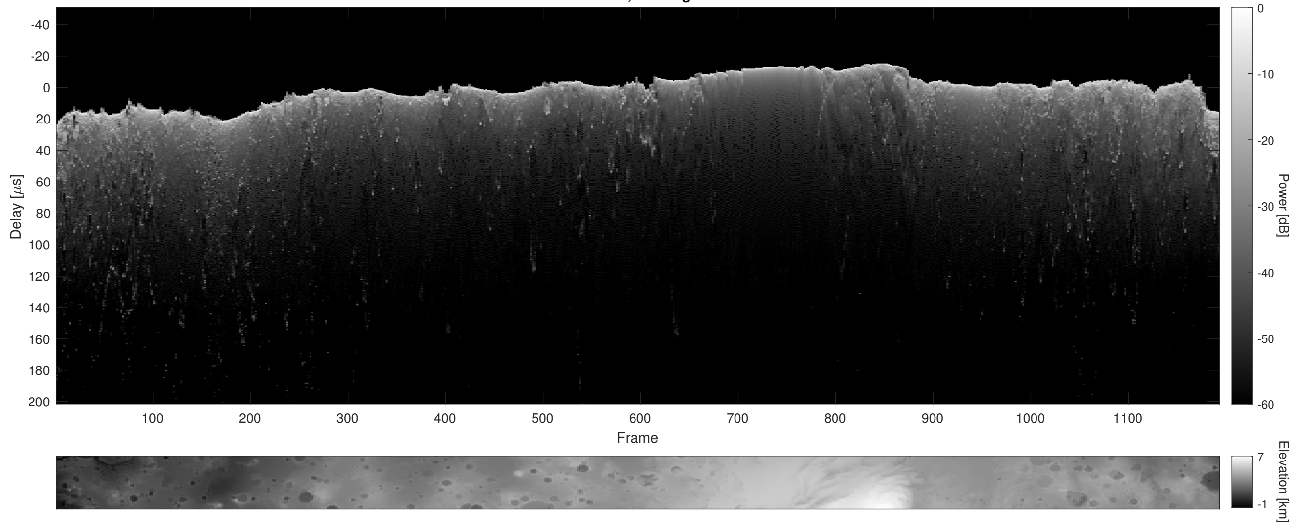
Orbit 8849, Cluttergram
