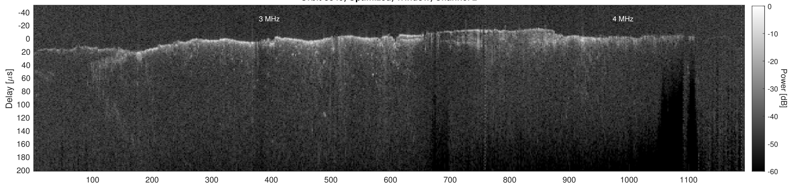
Orbit 8849, Cluttergram
