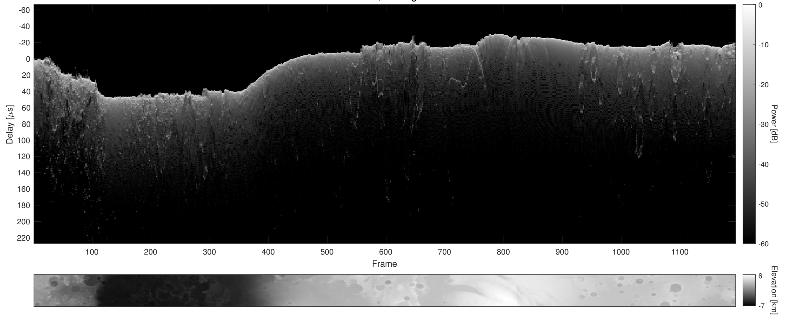
Orbit 8850, Cluttergram
